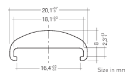
Semi-transparent 60° cover
